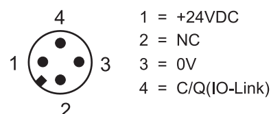
IO-Link M12 interface
