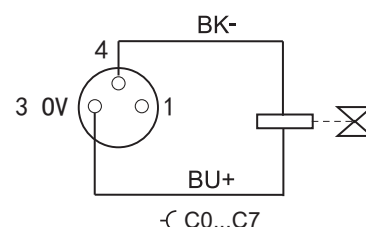
Digital I/O M8 interface
