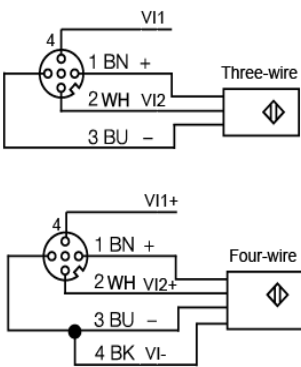
Sensor Connection
