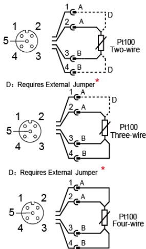
RTD Connection
