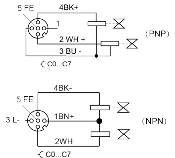
Digital output M12 interface
