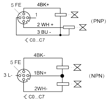
Digital output M12 interface
