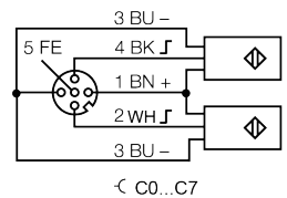
Digital input M12 interface
