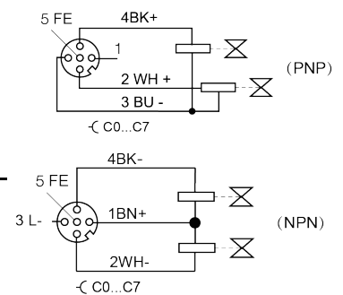
Digital output M12 interface
