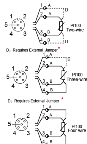
RTD Connection
