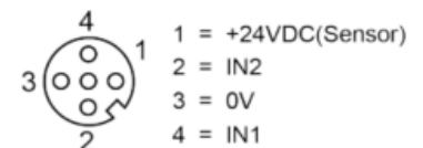
Input signal connection M12
