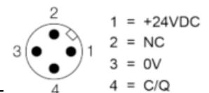
Input signal connection M12
